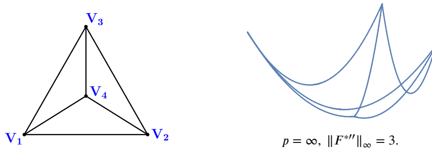
Figure 2 Example 1: (left) the triangulation T ; (right) the corresponding edge convex minimum L_{\infty} -norm network F^*
